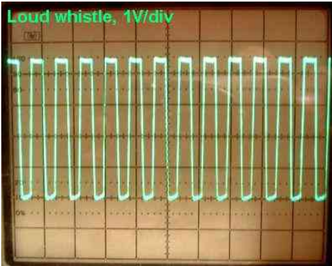
Loud whistle, about 10cm from microphone. Vertical scale is 1V/division, so the display shows 0 - 8V, m
